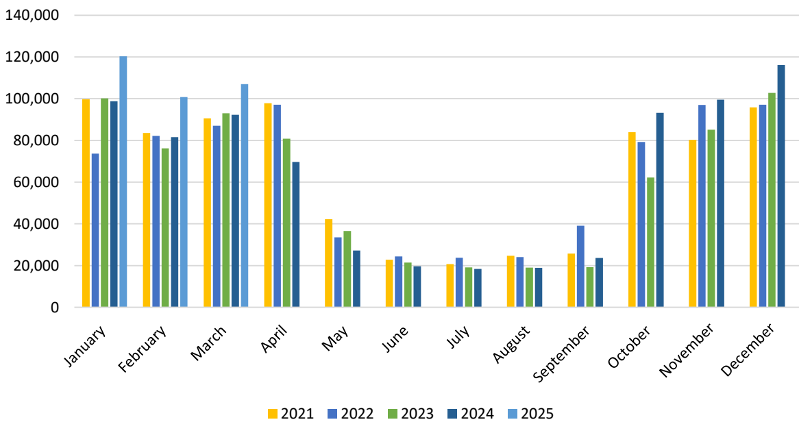
Figure 4 Volume of heat sold in Miskolc (GJ)
